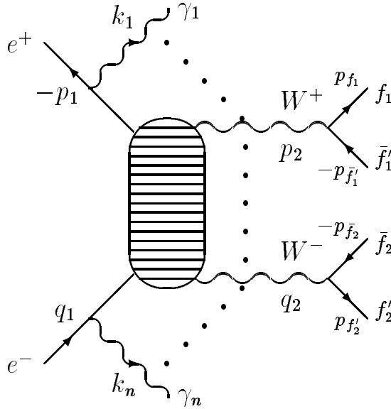
Figure 1: The process e^+e^- \rightarrow W^+W^- \rightarrow 4fermions = f_1 + \bar{f}'_1 + \bar{f}_2 + f'_2 , where \begin{pmatrix} f_i \\ f'_i \end{pmatrix}_L \equiv \frac{1}{2}(1 - \gamma_5) \begin{pmatrix} f_i \\ f'_i \end{pmatrix} , i = 1, 2 , are SU_{2L} doublets. Here, p_A is the 4-momentum of A , A = f_i, f'_i, p_1(q_1) and p_2(q_2) are the 4-momenta of e^+(e^-) and W^+(W^-) respectively.
