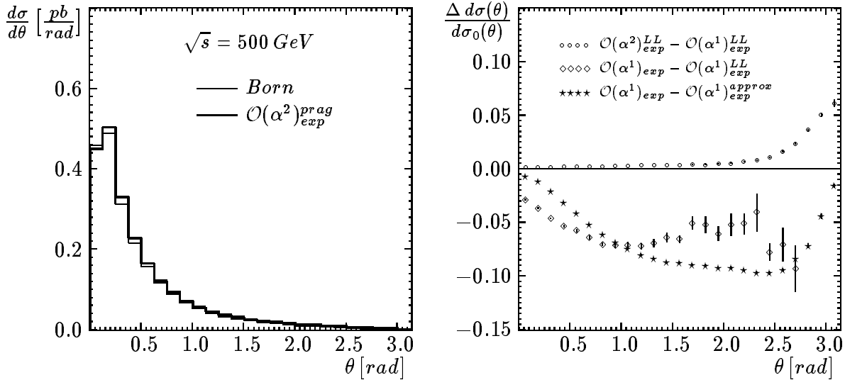
Figure 4: The same as in Fig. 2 but for the NLC energy: \sqrt{s} = 500 GeV.
