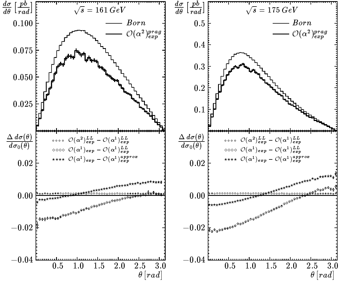
Figure 2: The W^- angular distributions for two LEP2 energies: \sqrt{s} = 161 GeV (left picture) and \sqrt{s} = 175 GeV (right picture). The upper parts of the pictures show the differential cross sections in Born (thin-lines) and in \mathcal{O}(\alpha^2)_{exp}^{prag} (thick-lines) approximations, where the latter one denotes the YFS exponentiated cross section including the exact \mathcal{O}(\alpha^1) matrix element together with the 2-nd order LL ISR terms (see the text for more details). In the lower part of each picture the following contributions to the YFS exponentiated cross section (divided by the corresponding Born differential cross section d\sigma_0 ) are presented: the 2-nd order LL ISR contribution ( \circ\circ ), the 1-st order non-LL contribution including electroweak radiative corrections ( \diamond\diamond ) and the difference between the exact \mathcal{O}(\alpha^1) matrix elements and the so-called Improved Born Approximation ( \star\star ). The last one shows the quality of IBA for the differential cross section as a function of the W -boson polar angle.
