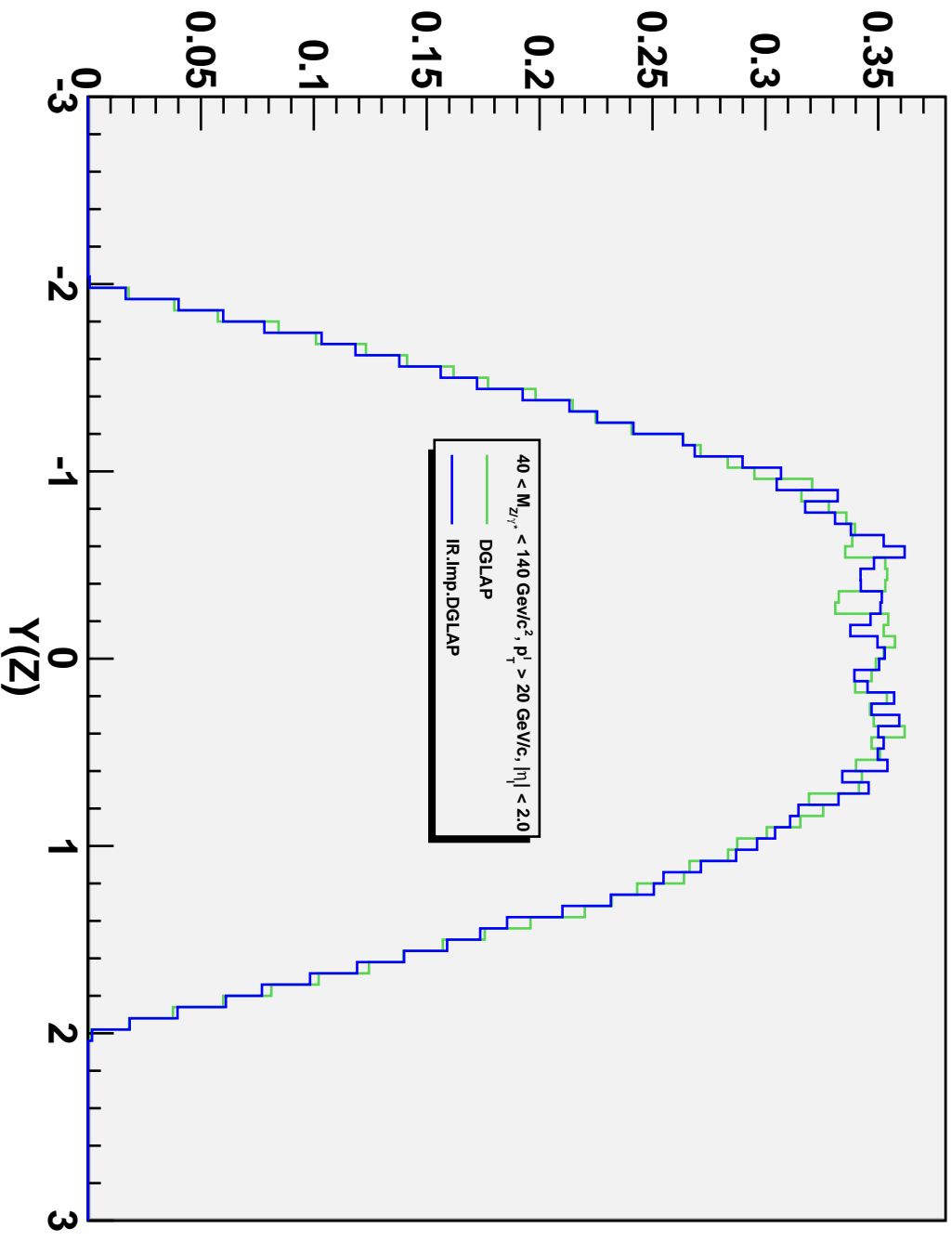
The unit normalized differential cross section for Z production as a function of vector boson rapidity.
